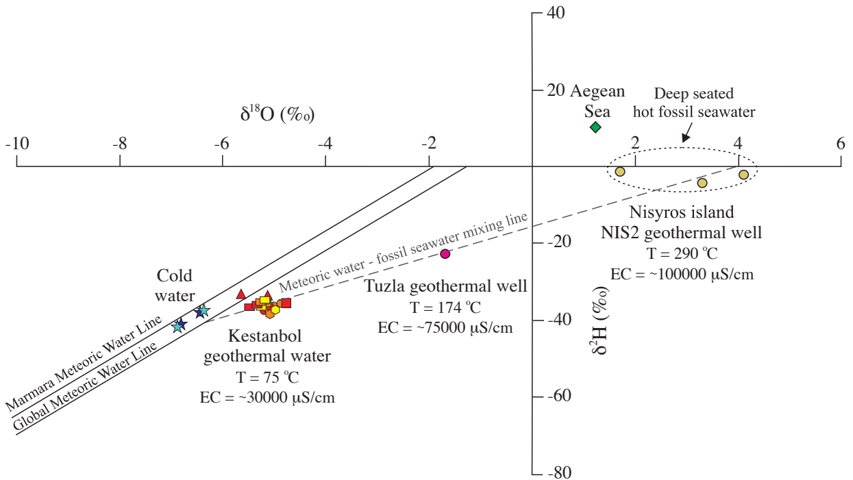
Figure 7. The plot of \delta^{18}\text{O} vs. \delta^2\text{H} (VSMOW) (modified from Yalcin, 2007).
