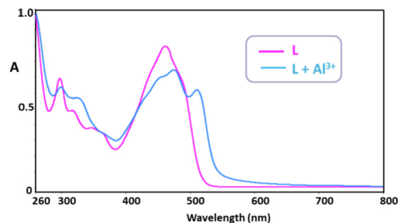
Fig. 1 UV-vis absorption spectra of L (0.1 mM) and L + \text{Al}^{3+} (0.5 mM) in EtOH.
