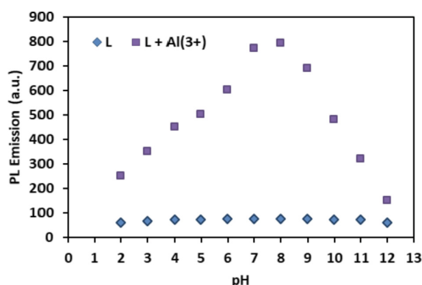
Fig. 3 pH dependence of L and L + \text{Al}^{3+} .
