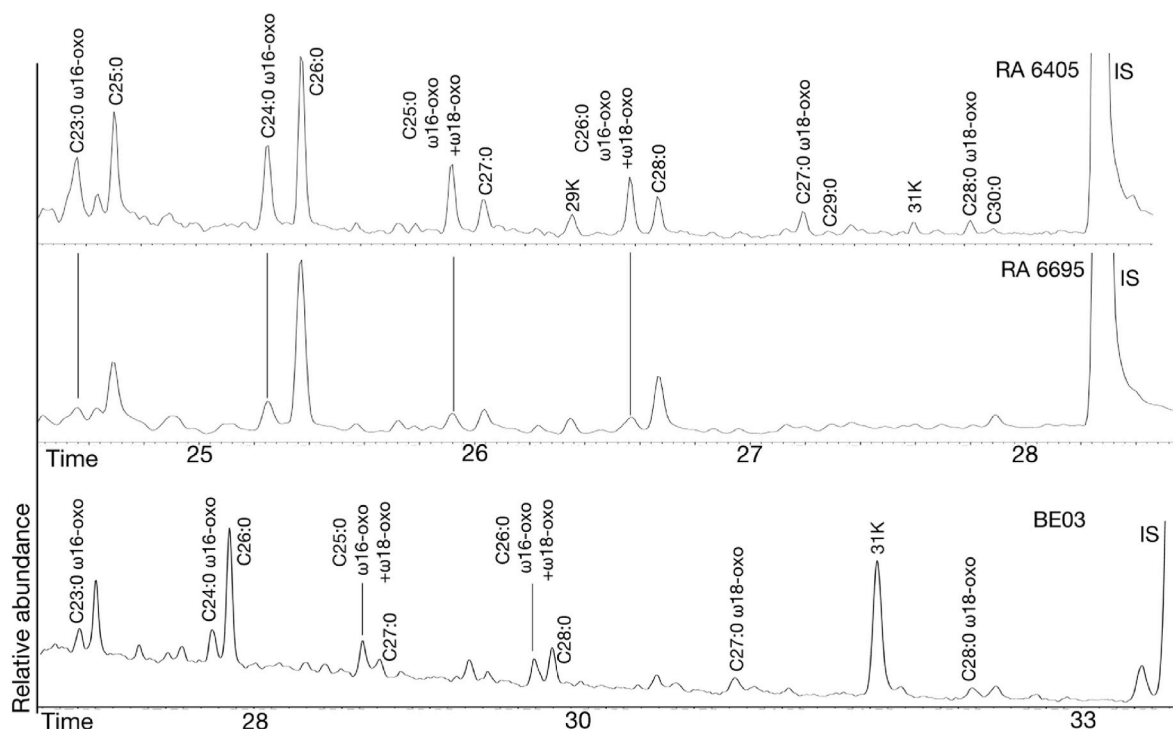
Fig. 5. GC-MS chromatograms showing the presence of oxoVLCFAs in samples from Carrer Reina Amàlia. Retention times in BE03 differ due to the use of different instrumentation (see SI2).
