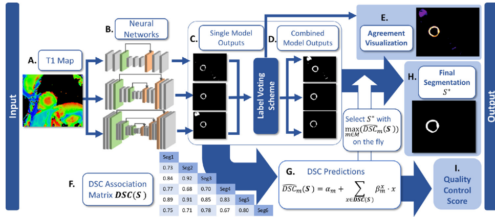
Fig. 1. Overview of the multiple neural network framework for integrated segmentation and quality control. For simplicity, this illustration shows an example of 3 single independent neural networks. (A) A T1 map is analyzed by (B) independent segmentation models to output (C) single-model segmentations. Then, the single-model segmentations are passed to a label voting scheme to generate (D) combined-model segmentations. (E) In addition, the agreement of the segmentation can be visualized. (F) A DSC matrix is generated from both single model and combined-model segmentations for (G) DSC predictions with regression models. (H) The final segmentation is chosen based on the DSC prediction, and the corresponding predicted DSC is output as (I) the final quality control score.
