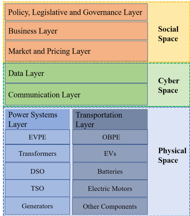
Figure 1: Cyber-Physical-Social Systems Layers of V2X
