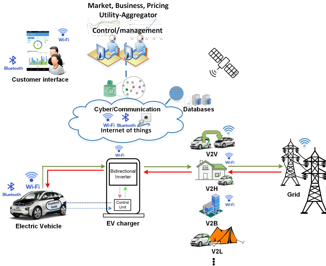
Figure 2: Cyber-Physical-Social Systems structure of V2X
