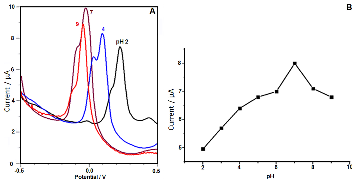
Figure 5. A) Differential pulse voltammograms of 5.0 \mu\text{M} compound 2 in BRBS with different pH values containing 0.1 M KCl and 30% DMF (pulse amplitude: 20 mV, pulse time: 30 s, scan rate: 25 \text{mV s}^{-1} ). B) Plot of peak current of compound 2 versus pH.
