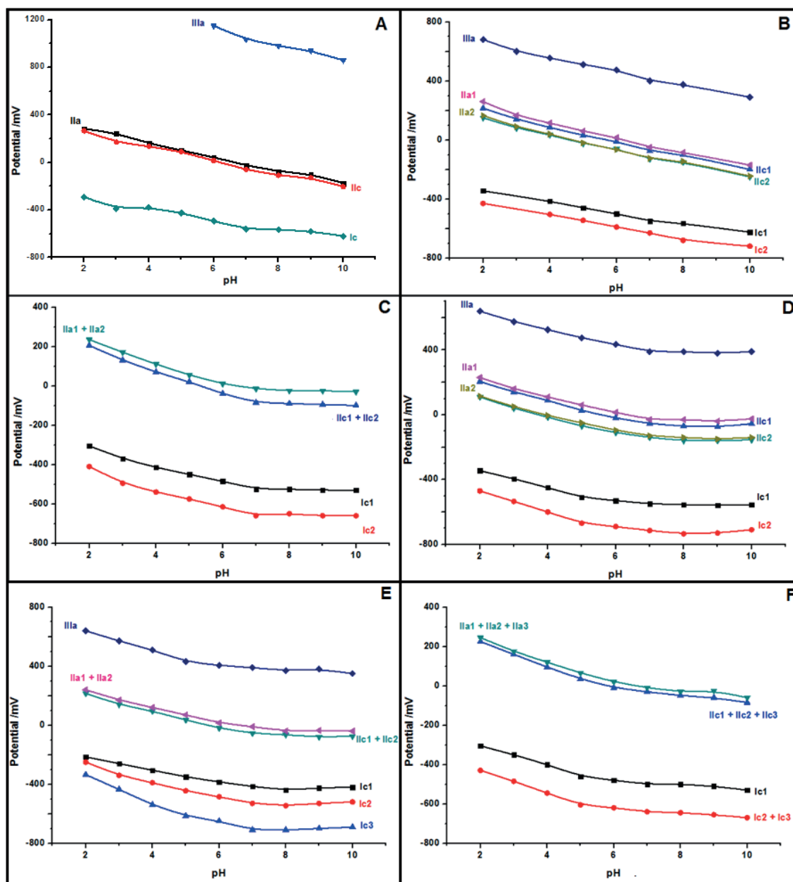
Figure S2. Plot of peak potentials of each nitro benzamide (compounds 1 (A), 2 (B), 3 (C), 4 (D), 5 (E), and 6 (F)) versus pH.
